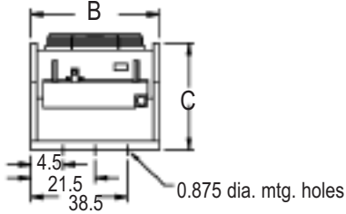
End View SMCR 15 - 40 hp
