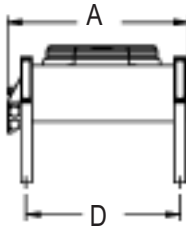
Side View SMCR 15 - 30 hp
