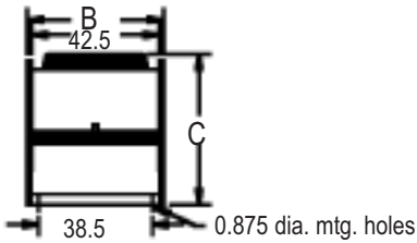
End View SMCR 15 - 40 hp
