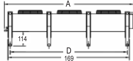
Side View SMCR 40 hp
