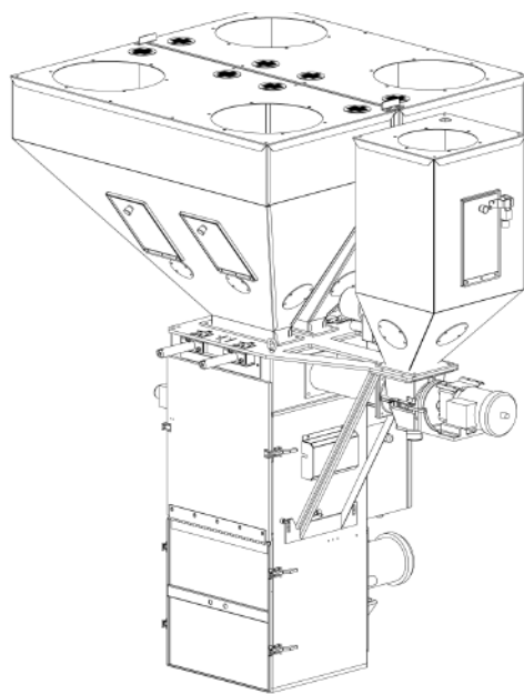
SGBD-2500-5R Includes: 4 Slidegates, 1 R.A.M. Hopper
