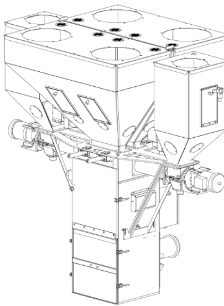
SGBD-2500-6RR Includes: 4 Slidegates, 2 R.A.M. Hoppers
