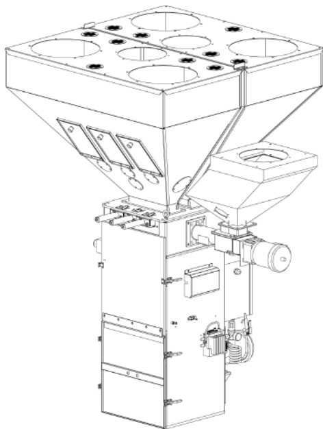
SGBD-2500-7F Includes: 6 Slidegates, 1 Additive Feeder
