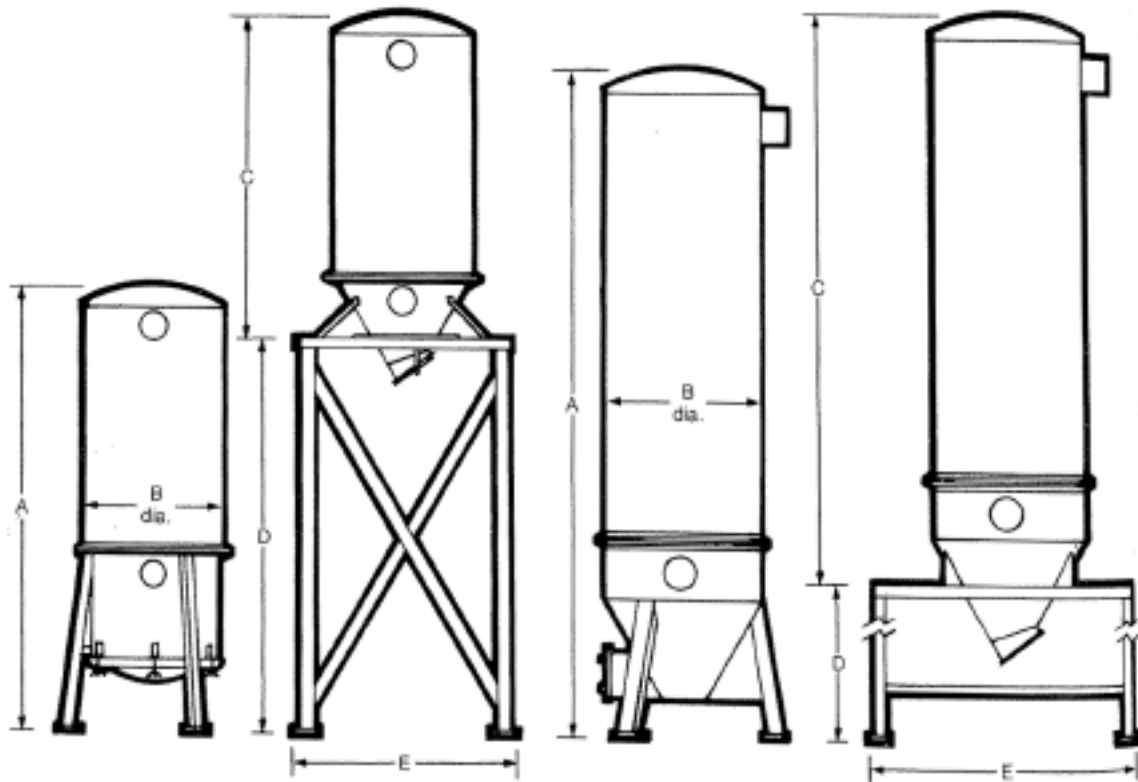
Floor Mount FC-15/FC-30
