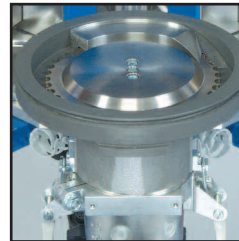
SDD 2 Feed Rate: 0.2-800 lbs/hr Operating Load: 0.4 kW Weight: 100lbs (45kg)
